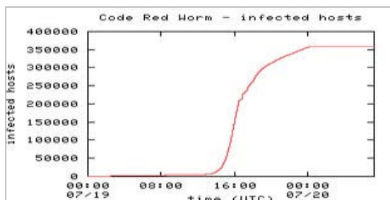
Fig. 4. Infected hosts by Code Red [10]
