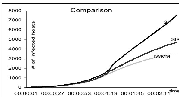
Fig. 3. Comparing SI, SIR and IWMM models
